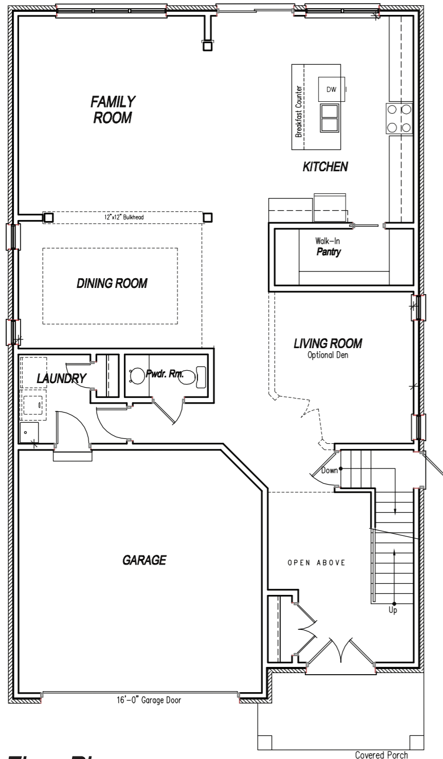
Main Floor Plan 1500 sq.ft. 9'-0" Main Floor Ceiling Height
