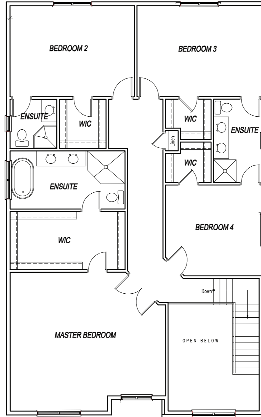
Second Floor Plan 1700 sq.ft. 8'-0" Second Floor Ceiling Height
