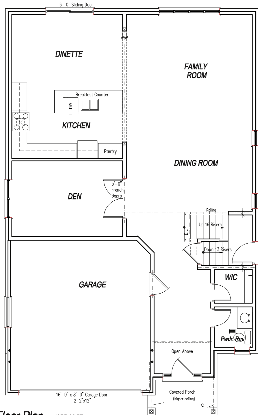
Main Floor Plan 1275 SQ.FT 9'-0" Main Floor Ceiling Height
