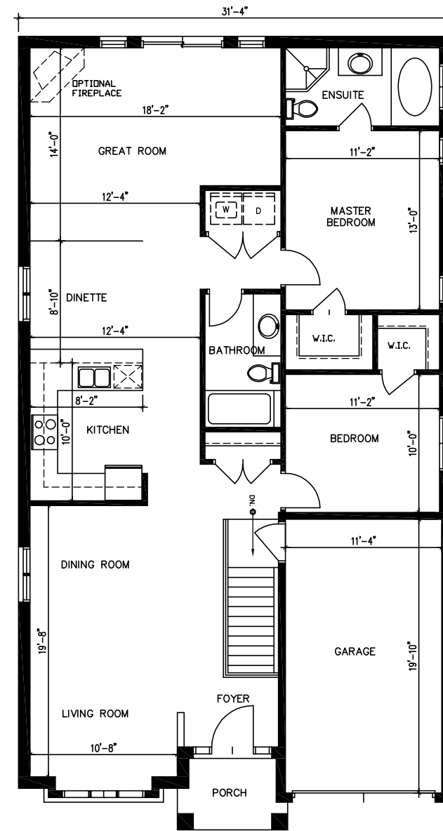
GROUND FLOOR 1468 S.F. TYPE "B"
