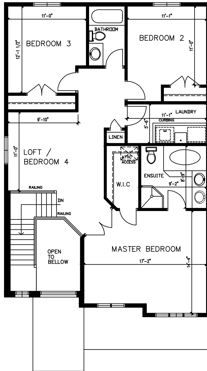
SECOND FLOOR 1221 s.f.
