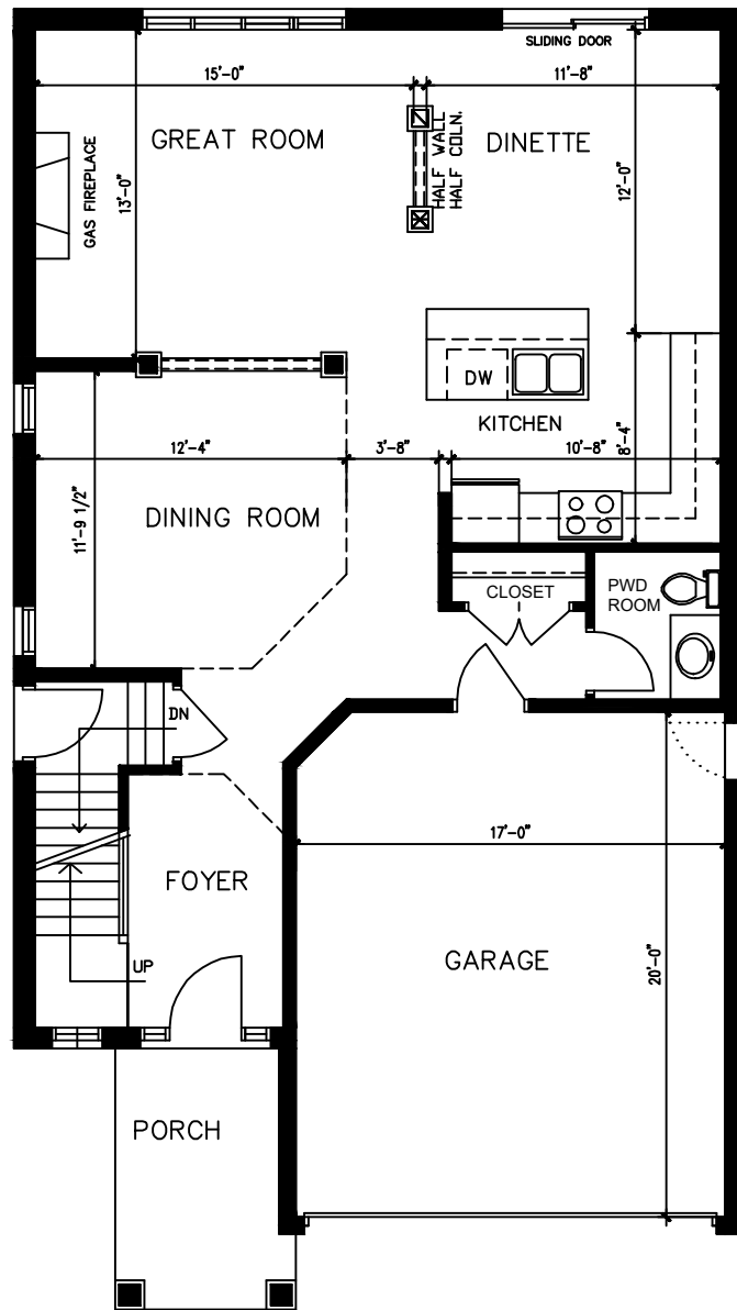
GROUND FLOOR 958 s.f.
